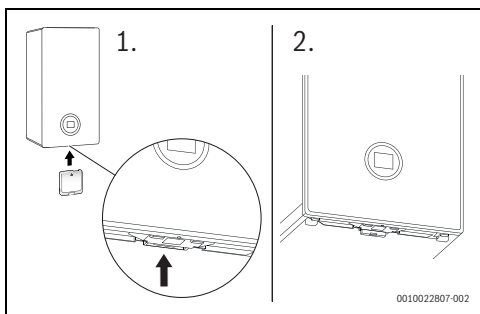
Obr. 3 Instalace Key
