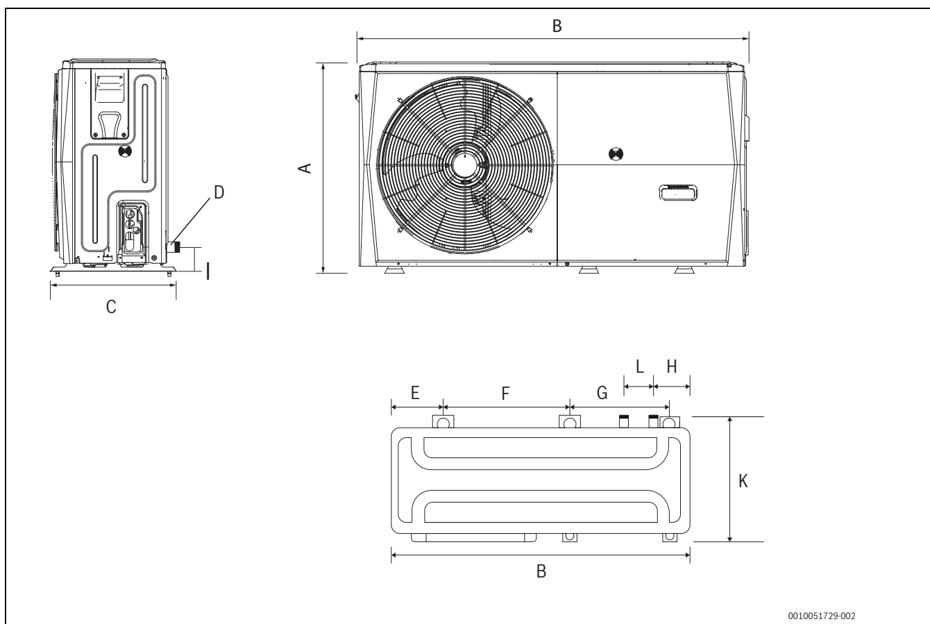
Obr. 32 Modely CS2000AWF 4 R-S až CS2000AWF 6 R-S
