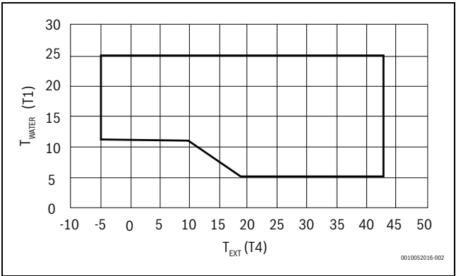
Obr. 11 CS2000AWF 4-6 R-S, CS2000AWF 8-10 R-S, CS2000AWF 12-16 R-S/T
