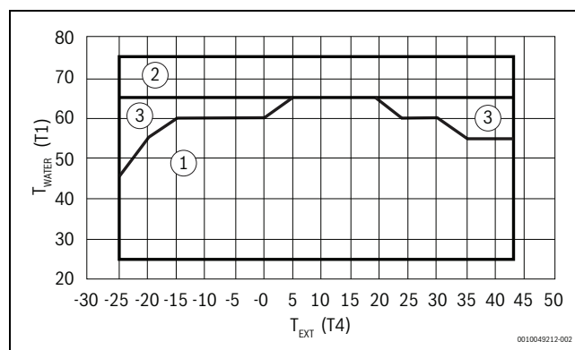
Obr. 9 CS2000AWF 4-6 R-S, CS2000AWF 8-10 R-S, CS2000AWF 12-16 R-S/T
