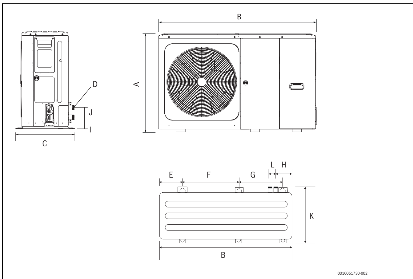
Obr. 33 Modely CS2000AWF 8 R-S až CS2000AWF 16 R-S/CS2000AWF 16 R-T
