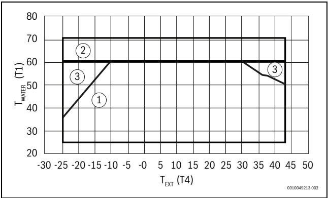
Obr. 10 CS2000AWF 18-30 R-T
