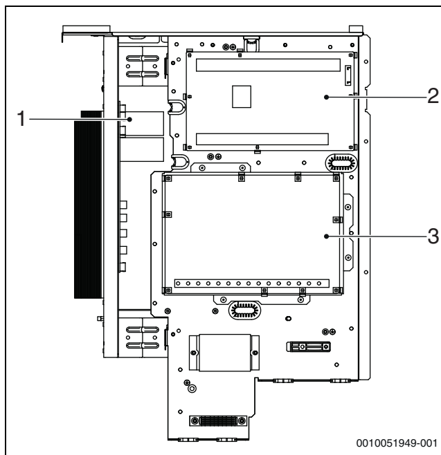
Obr. 63 Velikosti CS2000AWF 18 R-T až CS2000AWF 16 R-S/ CS2000AWF 30 R-T
