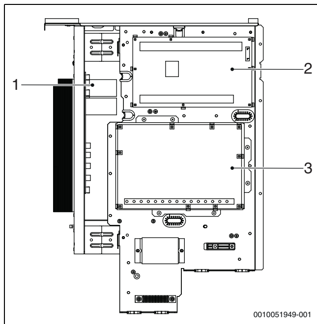
Obr. 62 Velikosti CS2000AWF 4 R-S až CS2000AWF 16 R-S/ CS2000AWF 16 R-T
