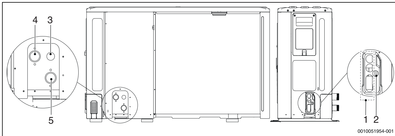
Obr. 65 Velikosti CS2000AWF 8 R-S až CS2000AWF 16 R-S/CS2000AWF 16 R-T
