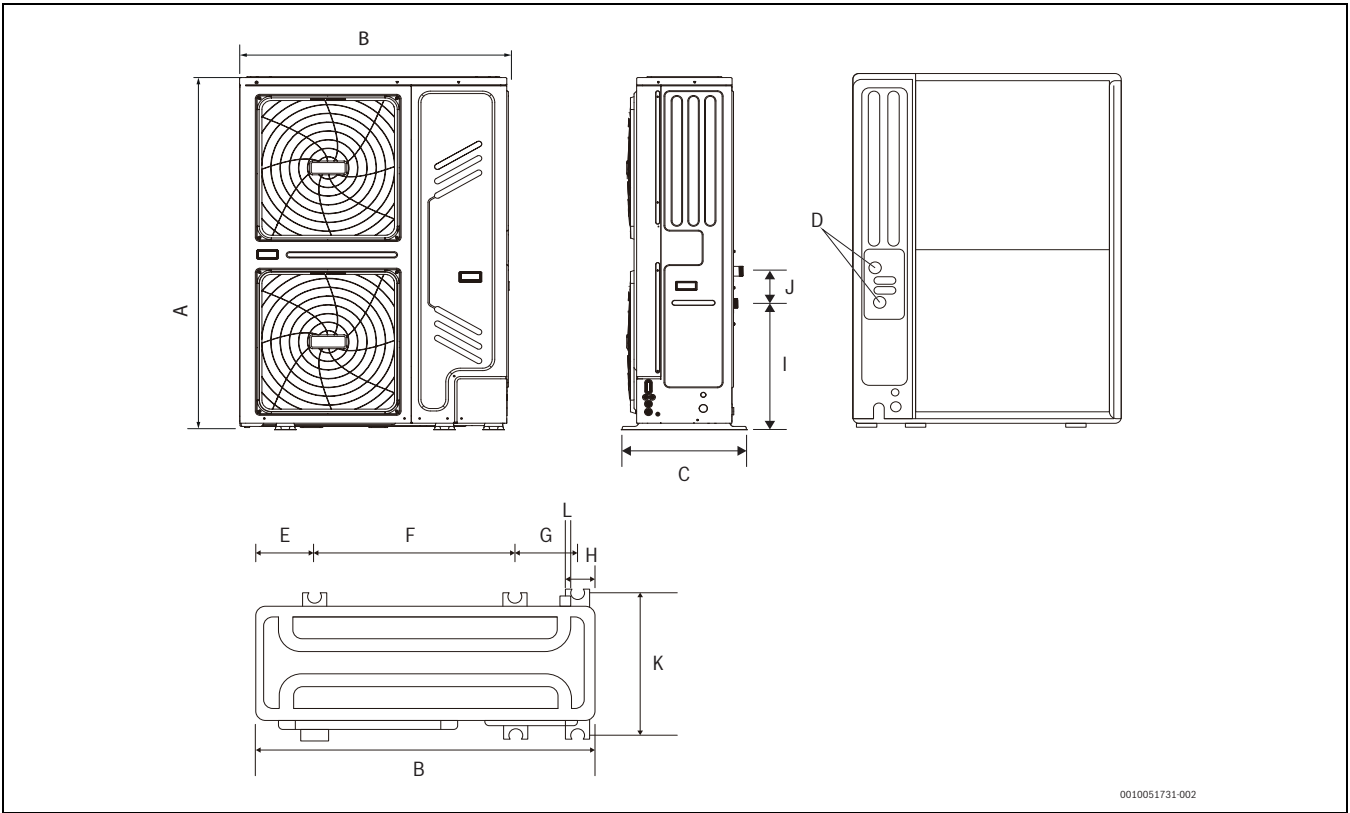
Obr. 34 Modely CS2000AWF 18 R-T až CS2000AWF 30 R-T
