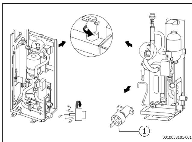
Obr. 55 Velikosti CS2000AWF 4 R-S–CS2000AWF 16 R-T/CS2000AWF 30 R-T
