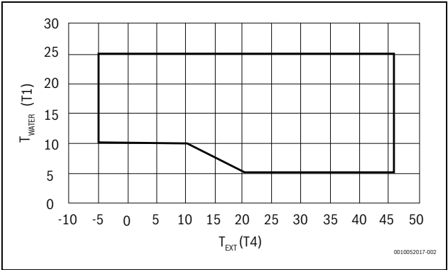
Obr. 12 CS2000AWF 18-30 R-T
