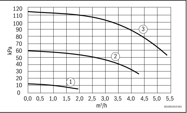
Obr. 14 CS2000AWF 18-30 R-T
