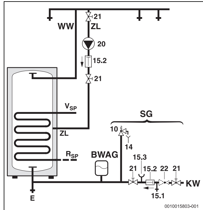
Fig. 2 Connection diagram on the domestic water side
